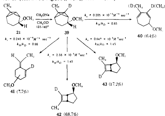
Chart IV. Synthesis and Ag^+ -Catalyzed Rearrangement Data for 39 (0.0924 M AgClO_4 , C_6H_6 , 40.0 \pm 0.1^\circ )
