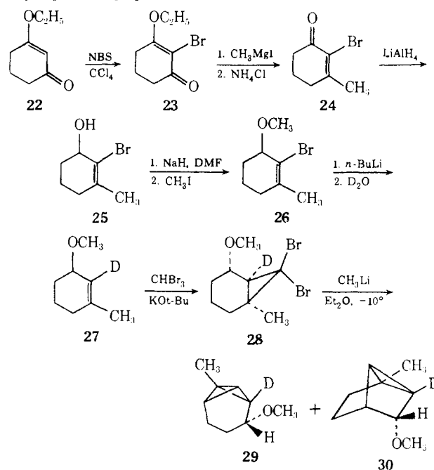
Chart II. Preparation of “Wing” Deuterium Labeled Tricyclo[4.1.0.0 2,7 ]heptane 29
