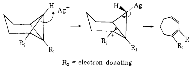
Chart V. A Detailed Mechanistic Interpretation of the Generalized Type \alpha Rearrangement
