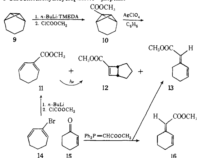
Chart I. Synthesis and Ag + -Catalyzed Rearrangement of 1-Carbomethoxytricyclo[4.1.0.0 2,7 ]heptane
