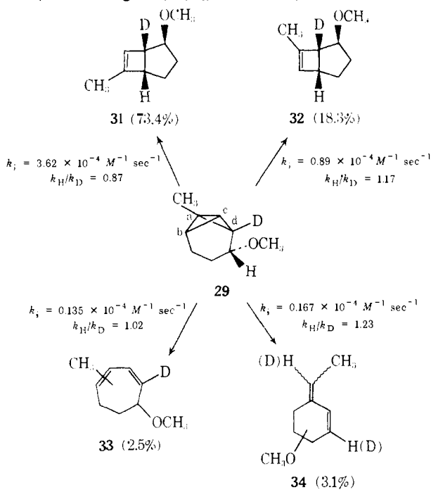
Chart III. Product Distribution, Catalytic Rate Constants, and Kinetic Deuterium Isotope Effects Arising from Rearrangement of 29 (0.0924 M AgClO 4 , C 6 H 6 , 40.0 \pm 0.1°)
