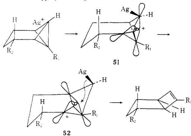
Chart VI. A Detailed Mechanistic Interpretation of the Generalized Type \gamma Rearrangement
